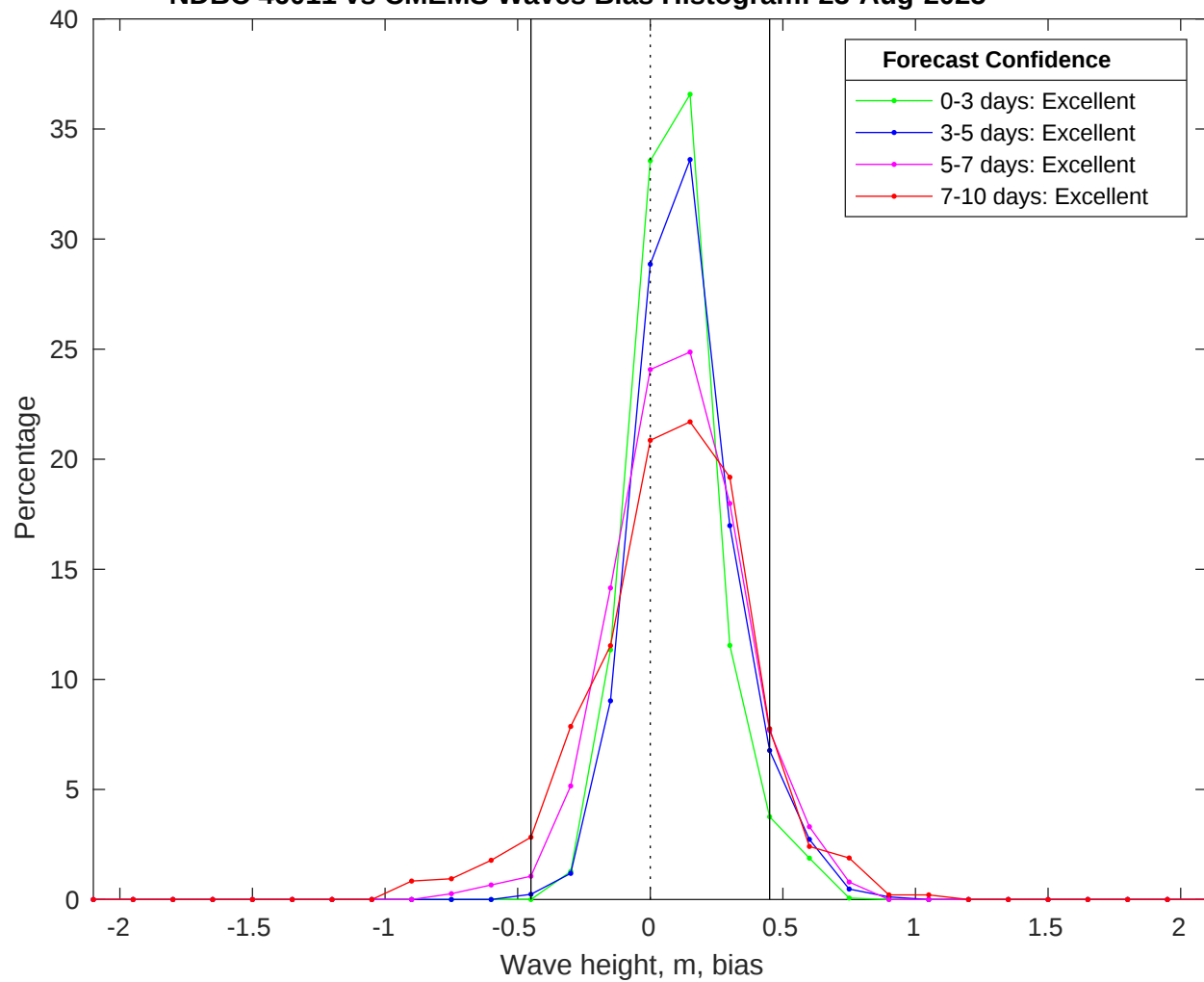
NDBC 46011 vs CMEMS Waves Bias Histogram: 23-Aug-2025
