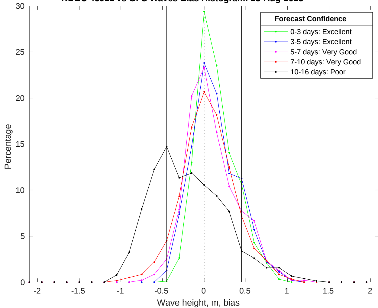
NDBC 46011 vs GFS Waves Bias Histogram: 23-Aug-2025
