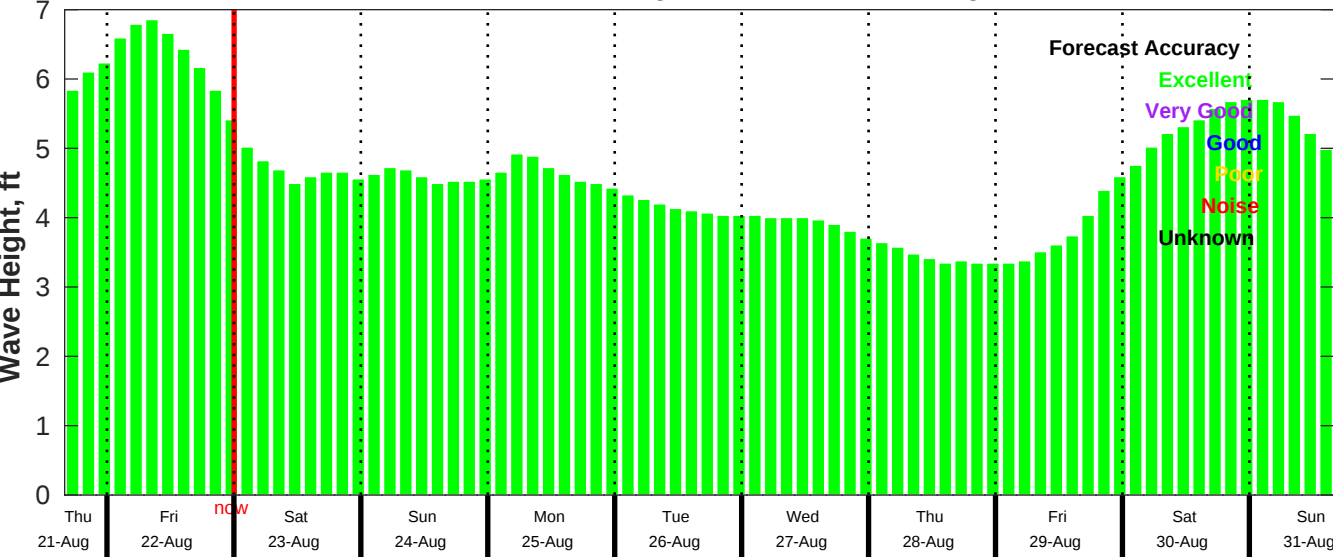
CMEMS Wave Forecast for NDBC 46011 from 21-Aug-2025 16:00:00 to 31-Aug-2025 16:00:00
