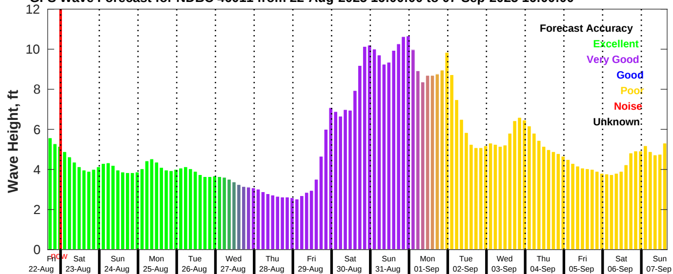
GFS Wave Forecast for NDBC 46011 from 22-Aug-2025 16:00:00 to 07-Sep-2025 16:00:00
