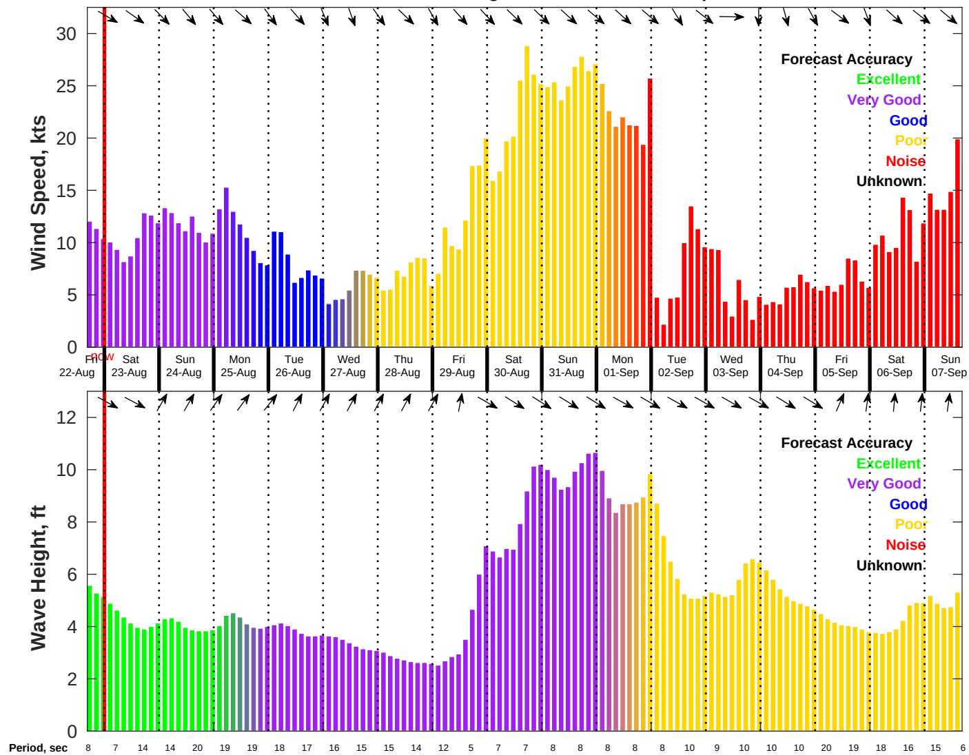
Wind & Wave Forecast for NDBC 46011 from 22-Aug-2025 16:00:00 to 07-Sep-2025 16:00:00
