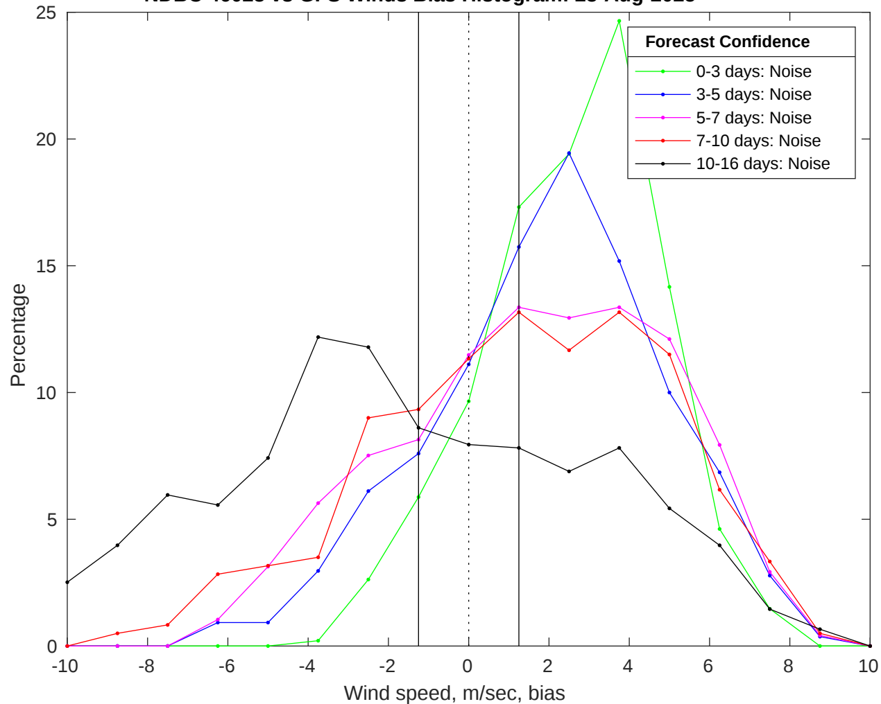
NDBC 46028 vs GFS Winds Bias Histogram: 23-Aug-2025
