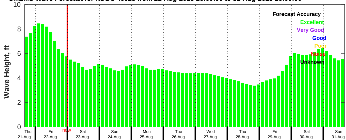
CMEMS Wave Forecast for NDBC 46028 from 21-Aug-2025 16:00:00 to 31-Aug-2025 16:00:00
