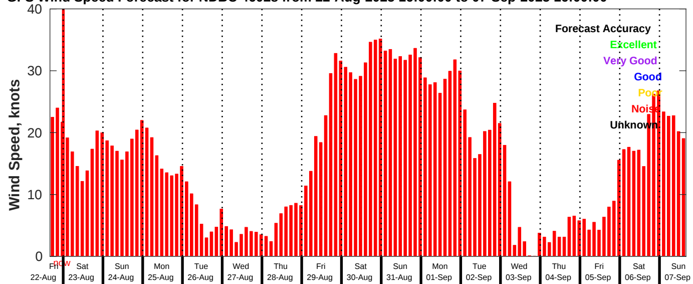
GFS Wind Speed Forecast for NDBC 46028 from 22-Aug-2025 16:00:00 to 07-Sep-2025 16:00:00
