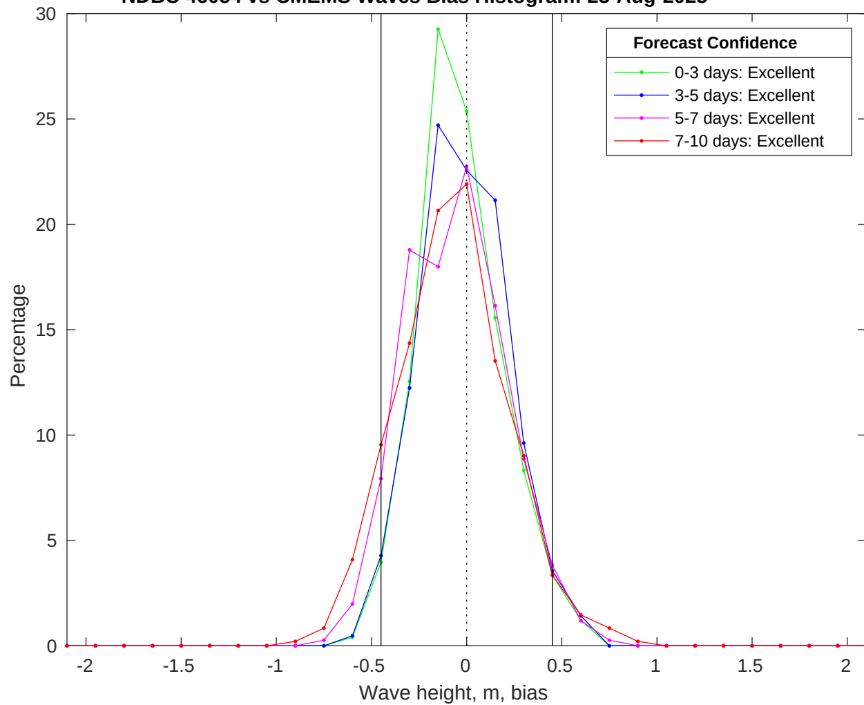
NDBC 46054 vs CMEMS Waves Bias Histogram: 23-Aug-2025
