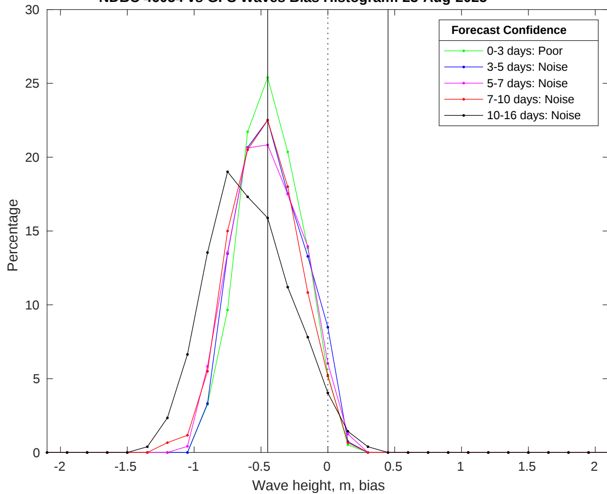
NDBC 46054 vs GFS Waves Bias Histogram: 23-Aug-2025
