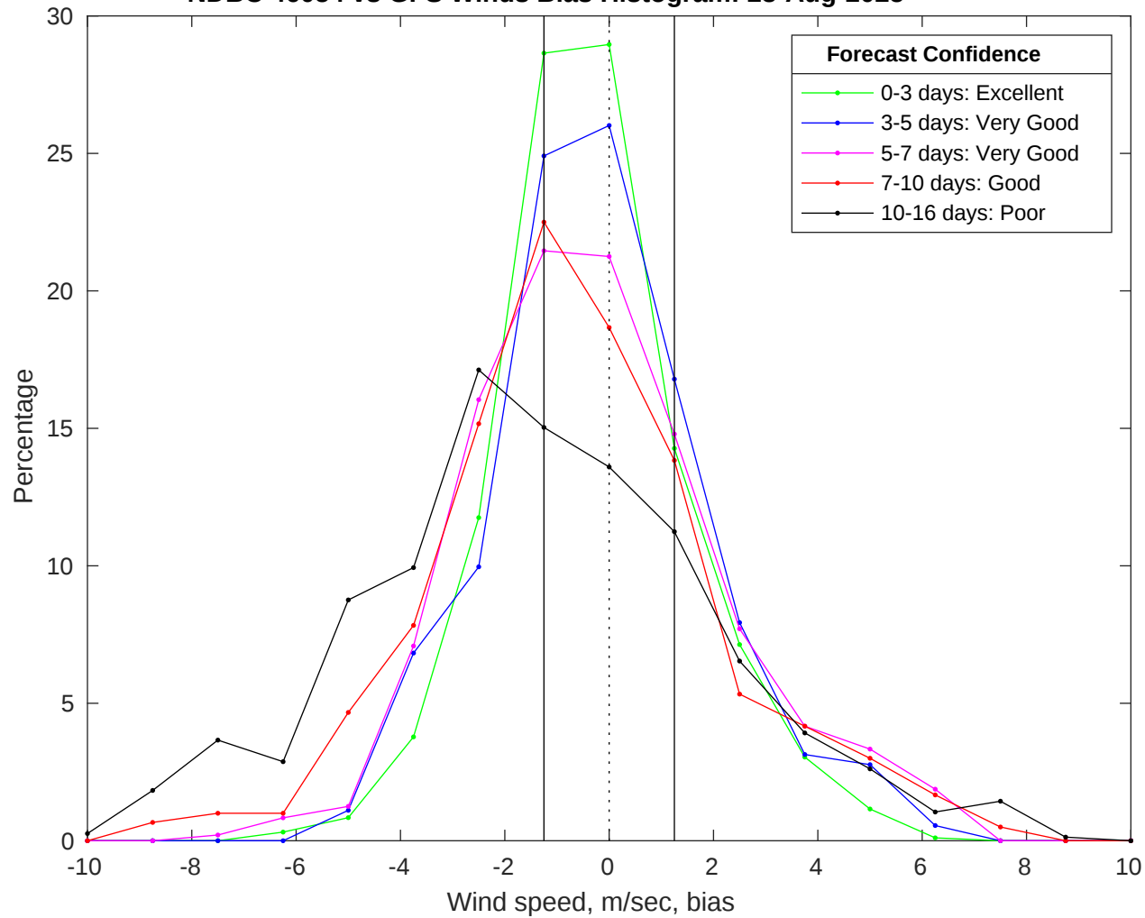
NDBC 46054 vs GFS Winds Bias Histogram: 23-Aug-2025
