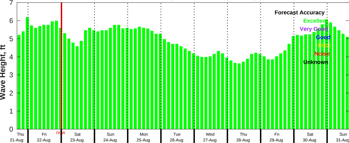
CMEMS Wave Forecast for NDBC 46054 from 21-Aug-2025 16:00:00 to 31-Aug-2025 16:00:00
