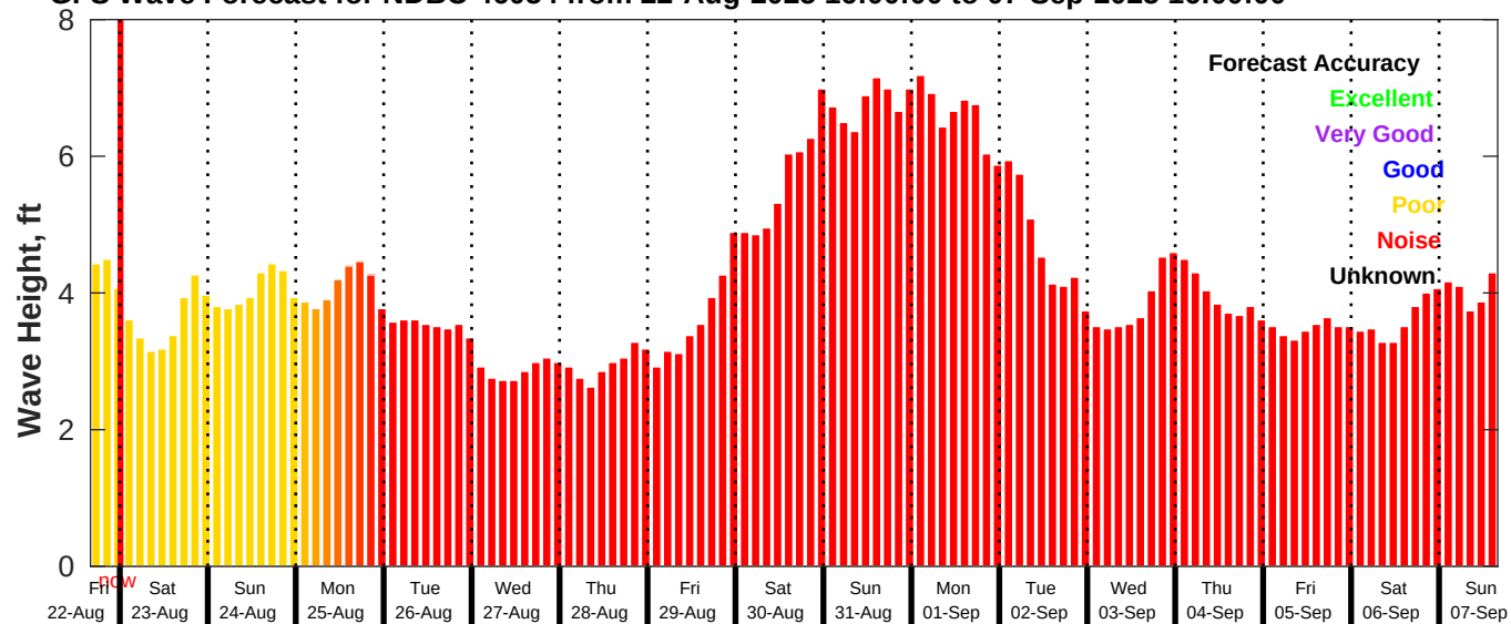
GFS Wave Forecast for NDBC 46054 from 22-Aug-2025 16:00:00 to 07-Sep-2025 16:00:00
