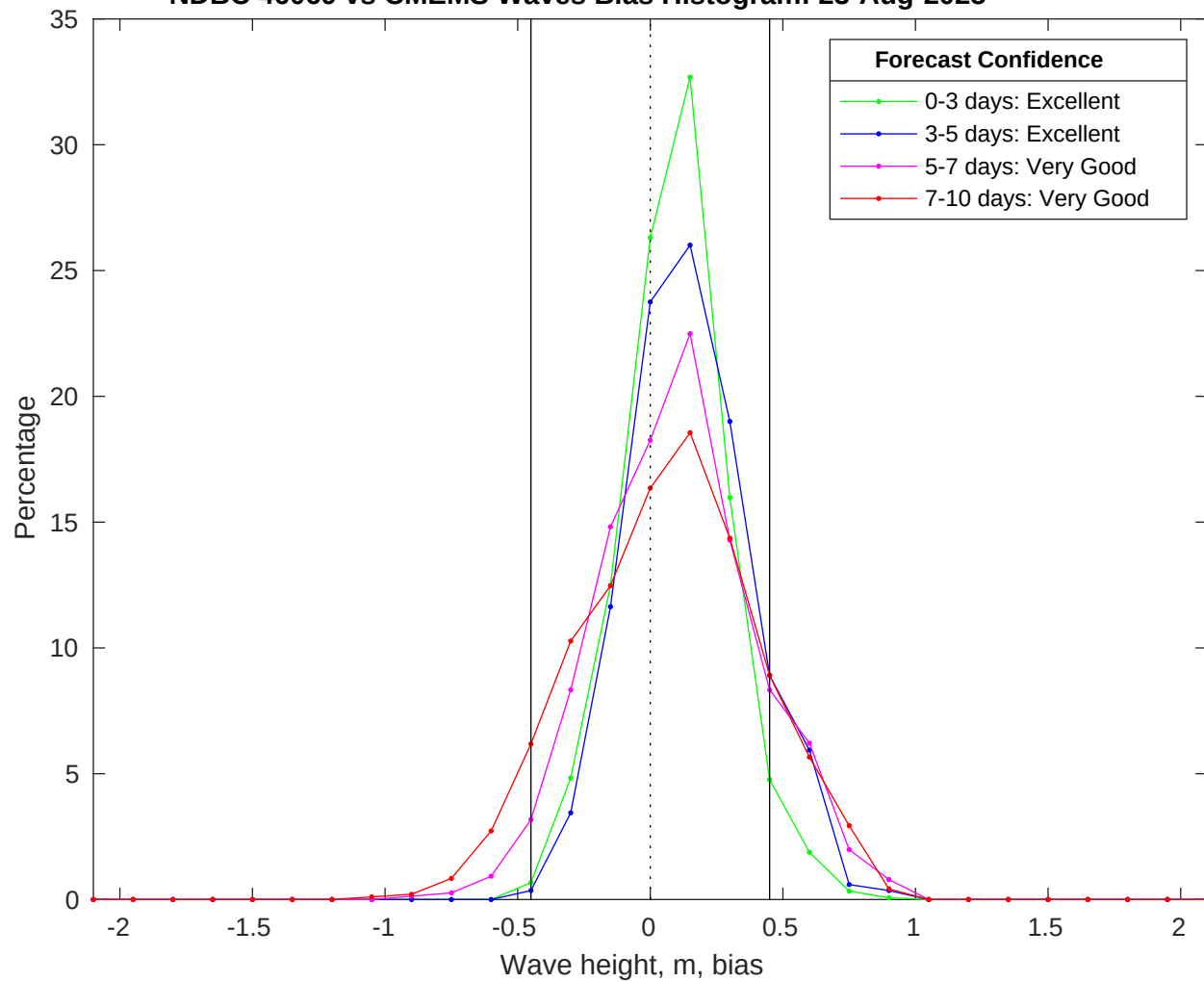
NDBC 46069 vs CMEMS Waves Bias Histogram: 23-Aug-2025
