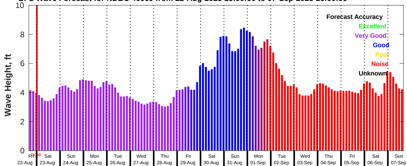
GFS Wave Forecast for NDBC 46069 from 22-Aug-2025 16:00:00 to 07-Sep-2025 16:00:00
