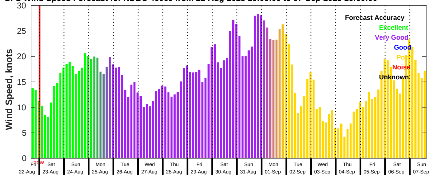
GFS Wind Speed Forecast for NDBC 46069 from 22-Aug-2025 16:00:00 to 07-Sep-2025 16:00:00
