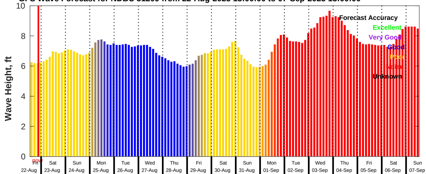
GFS Wave Forecast for NDBC 51209 from 22-Aug-2025 13:00:00 to 07-Sep-2025 13:00:00
