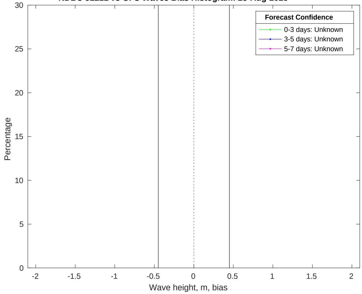
NDBC 51211 vs GFS Waves Bias Histogram: 23-Aug-2025
