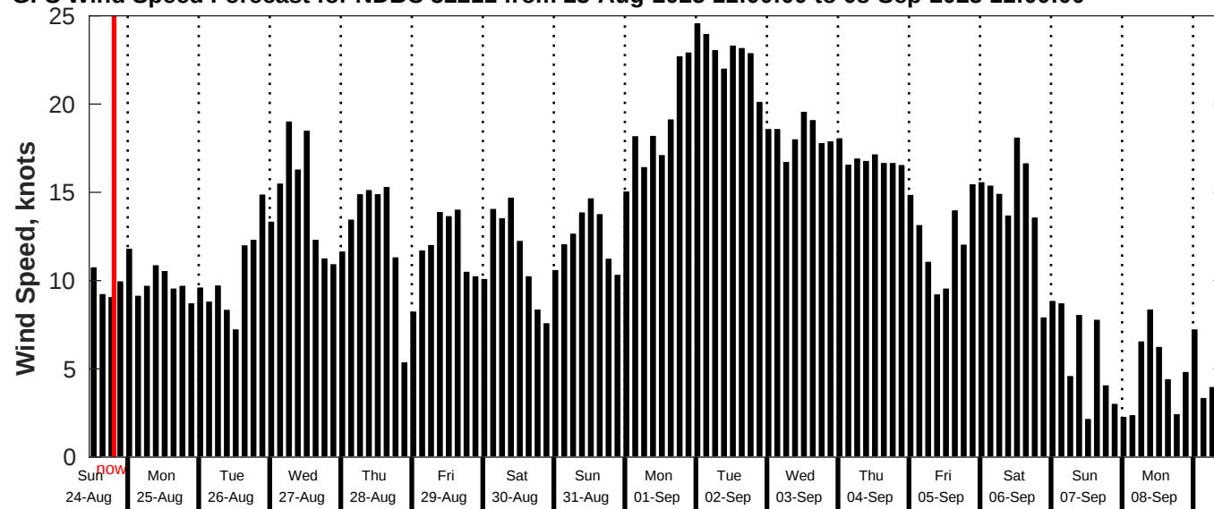
GFS Wind Speed Forecast for NDBC 52211 from 23-Aug-2025 11:00:00 to 08-Sep-2025 11:00:00
