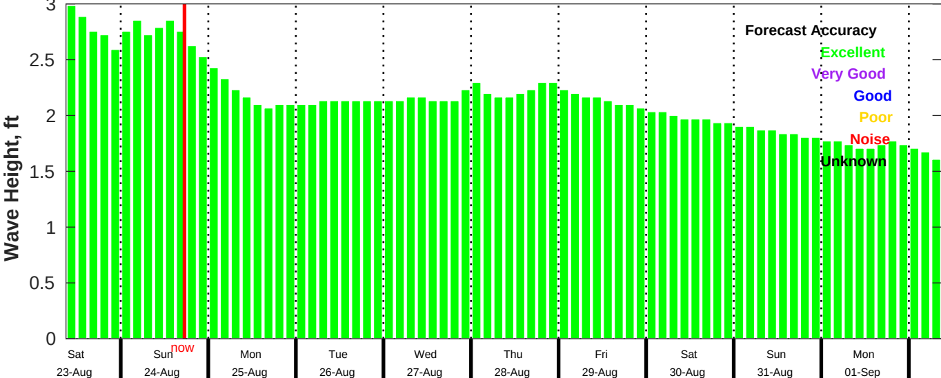
CMEMS Wave Forecast for NDBC 52212 from 22-Aug-2025 09:00:00 to 01-Sep-2025 09:00:00
