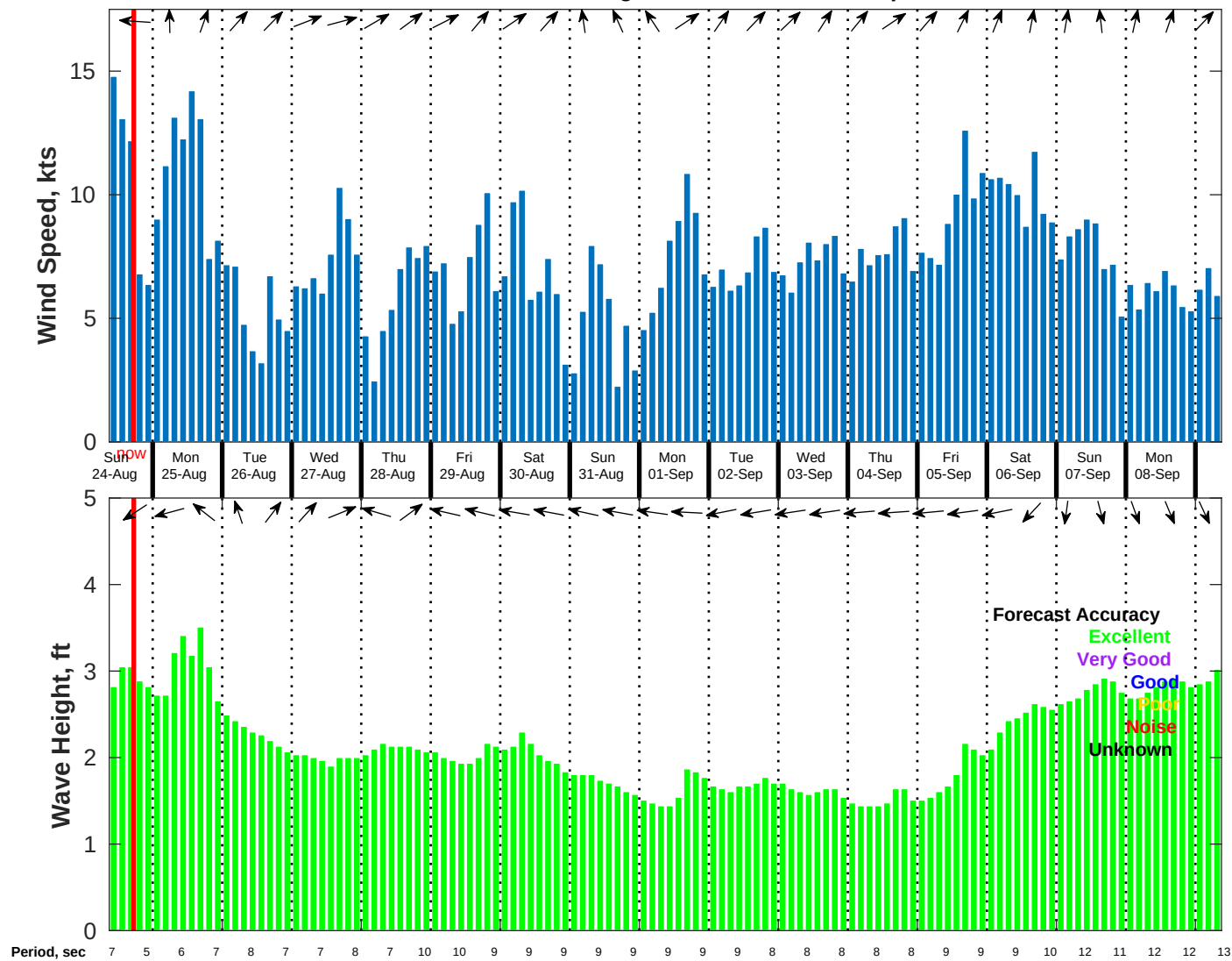
Wind & Wave Forecast for NDBC 52212 from 23-Aug-2025 09:00:00 to 08-Sep-2025 09:00:00
