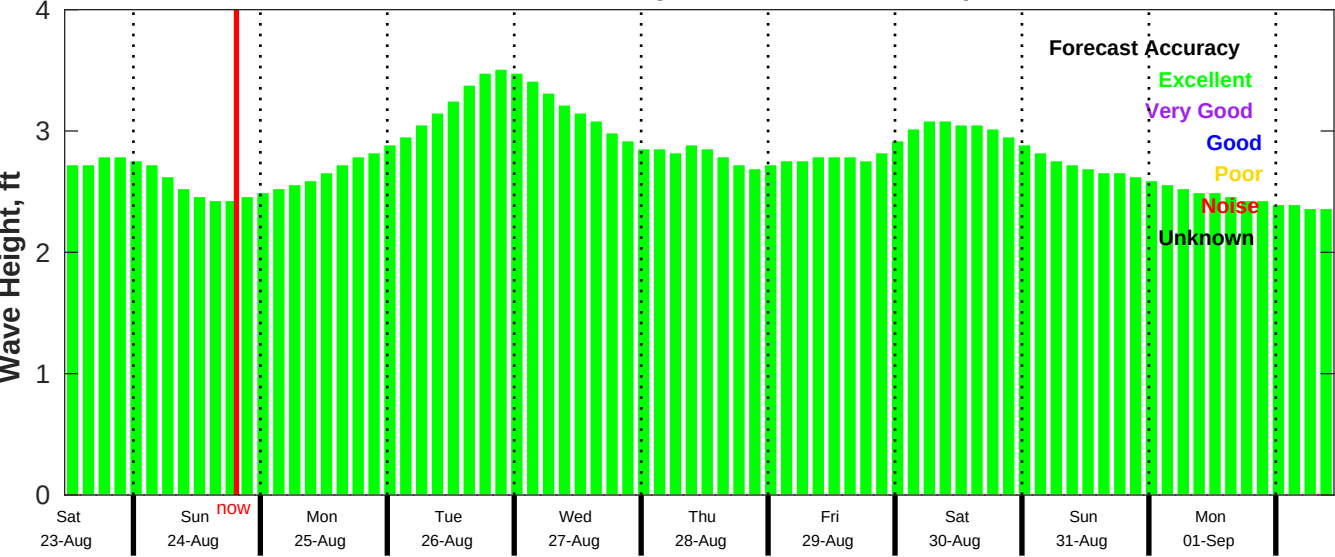
CMEMS Wave Forecast for NDBC 52213 from 22-Aug-2025 11:00:00 to 01-Sep-2025 11:00:00
