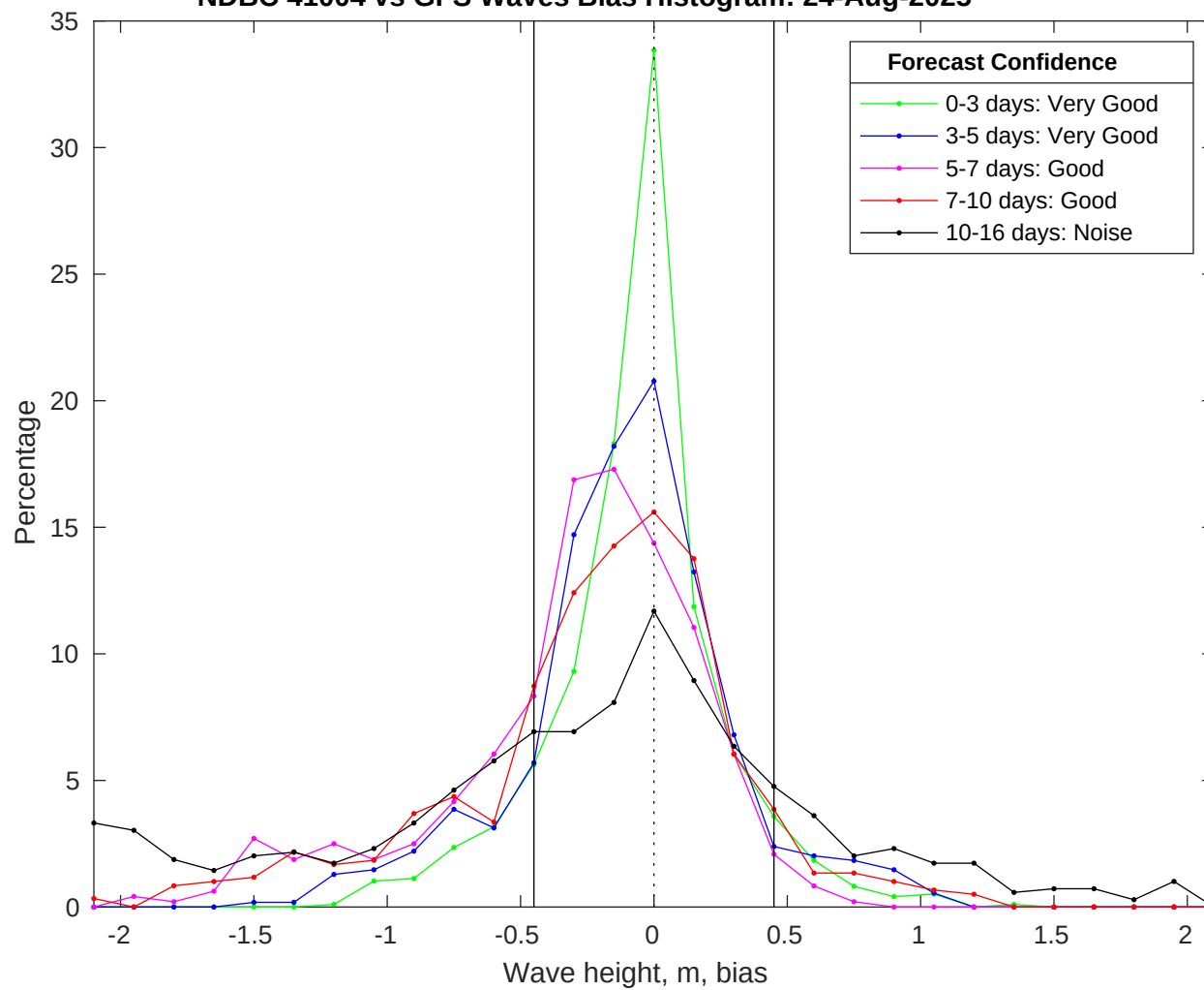
NDBC 41004 vs GFS Waves Bias Histogram: 24-Aug-2025
