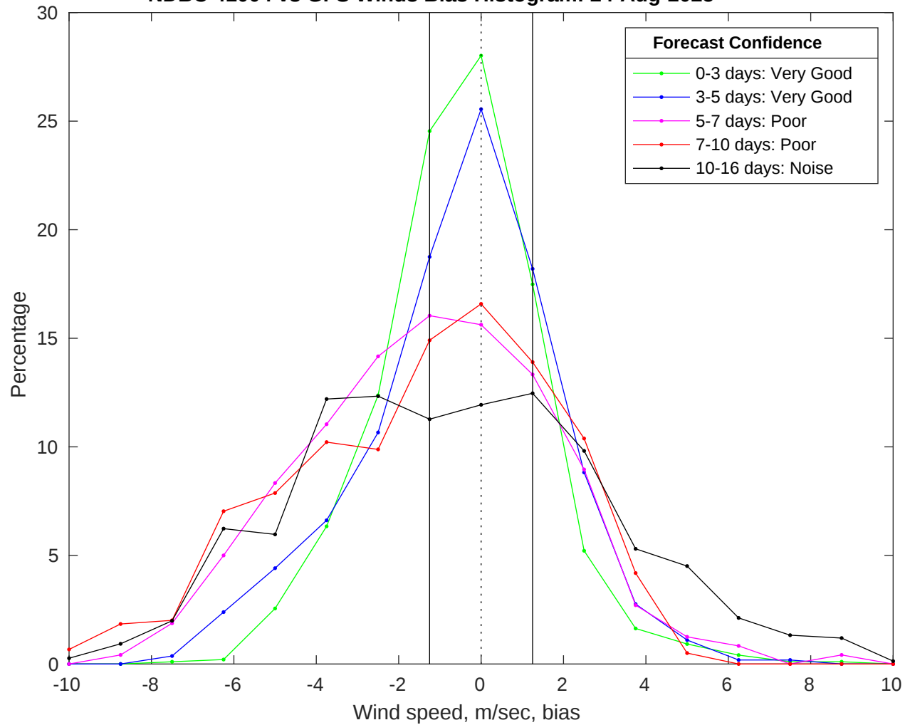
NDBC 41004 vs GFS Winds Bias Histogram: 24-Aug-2025
