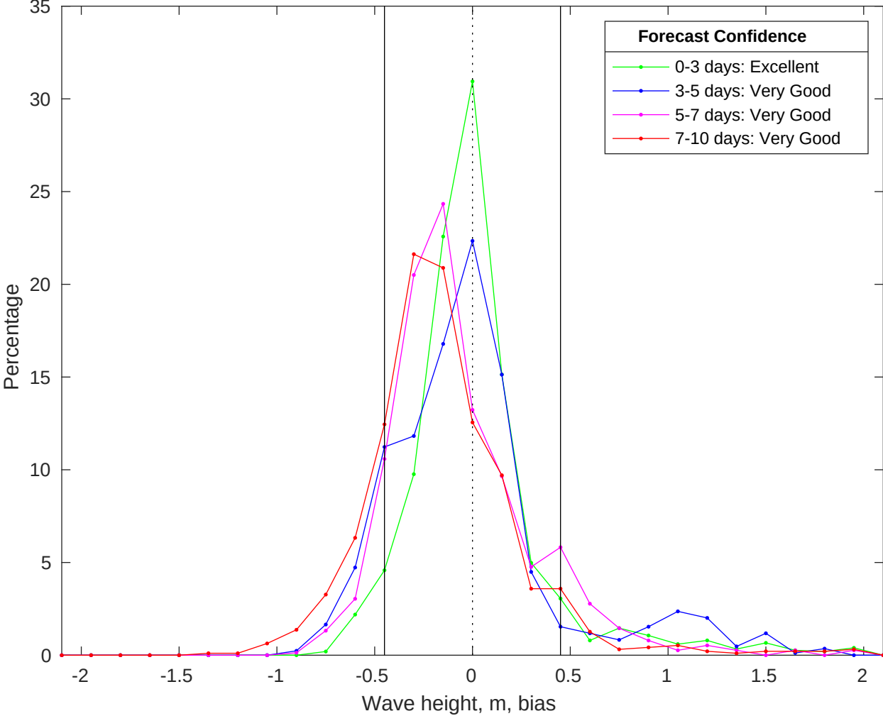
NDBC 41013 vs CMEMS Waves Bias Histogram: 24-Aug-2025
