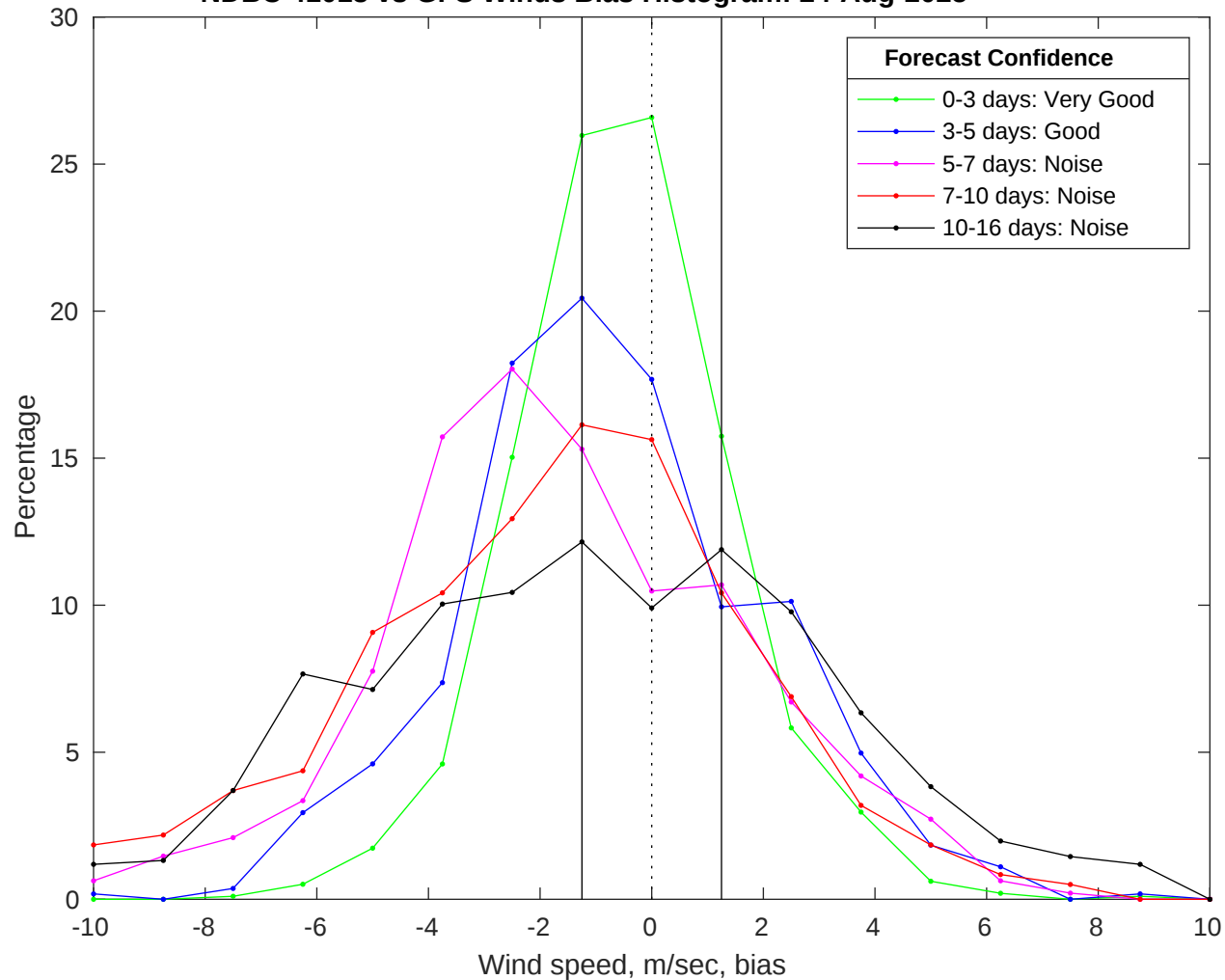
NDBC 41013 vs GFS Winds Bias Histogram: 24-Aug-2025
