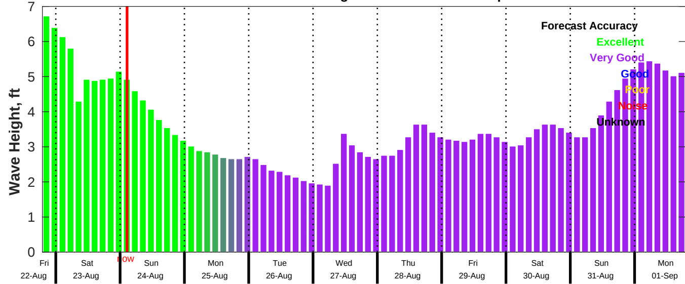
CMEMS Wave Forecast for NDBC 41013 from 22-Aug-2025 19:00:00 to 01-Sep-2025 19:00:00
