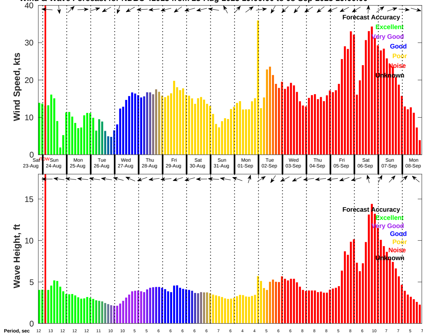
Wind & Wave Forecast for NDBC 41013 from 23-Aug-2025 19:00:00 to 08-Sep-2025 19:00:00
