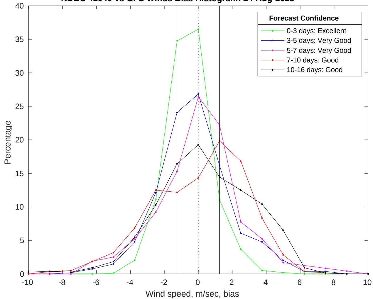
NDBC 41040 vs GFS Winds Bias Histogram: 24-Aug-2025
