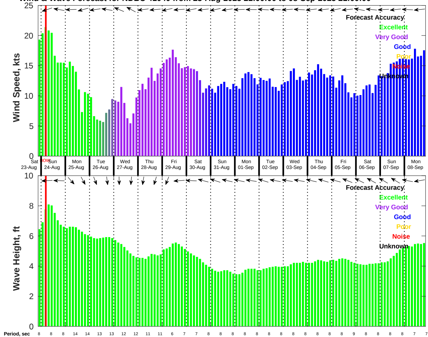
Wind & Wave Forecast for NDBC 41040 from 23-Aug-2025 21:00:00 to 08-Sep-2025 21:00:00
