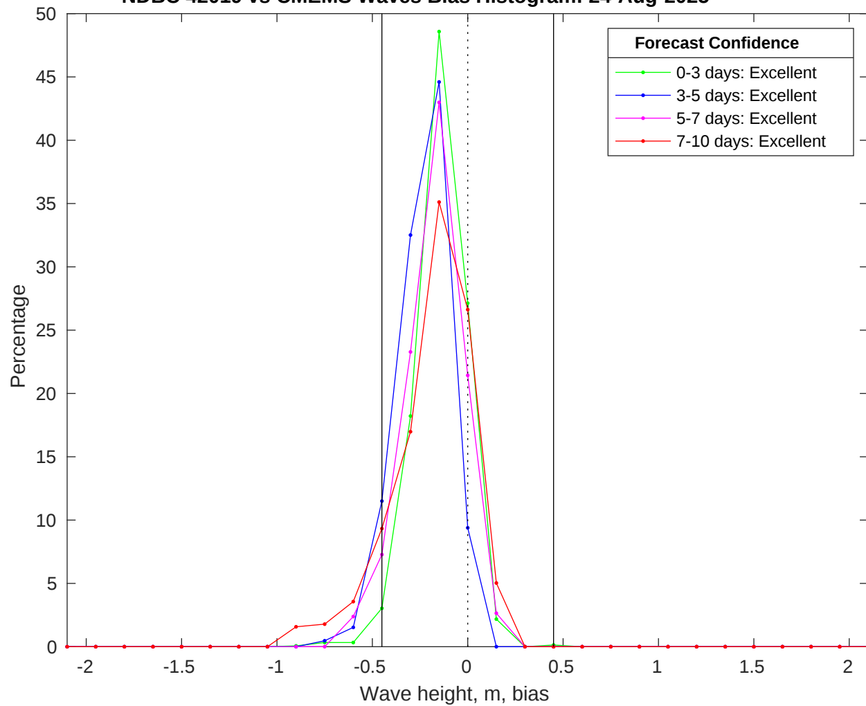
NDBC 42019 vs CMEMS Waves Bias Histogram: 24-Aug-2025
