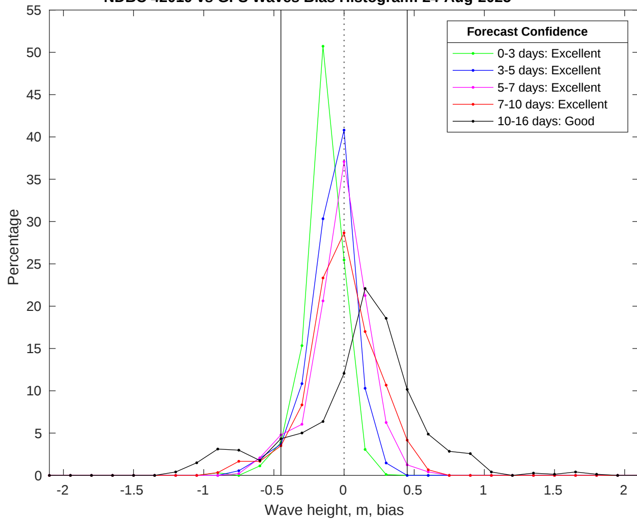
NDBC 42019 vs GFS Waves Bias Histogram: 24-Aug-2025
