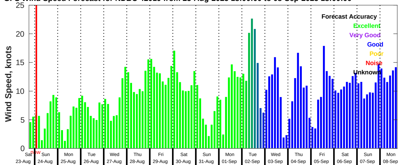
GFS Wind Speed Forecast for NDBC 42019 from 23-Aug-2025 18:00:00 to 08-Sep-2025 18:00:00
