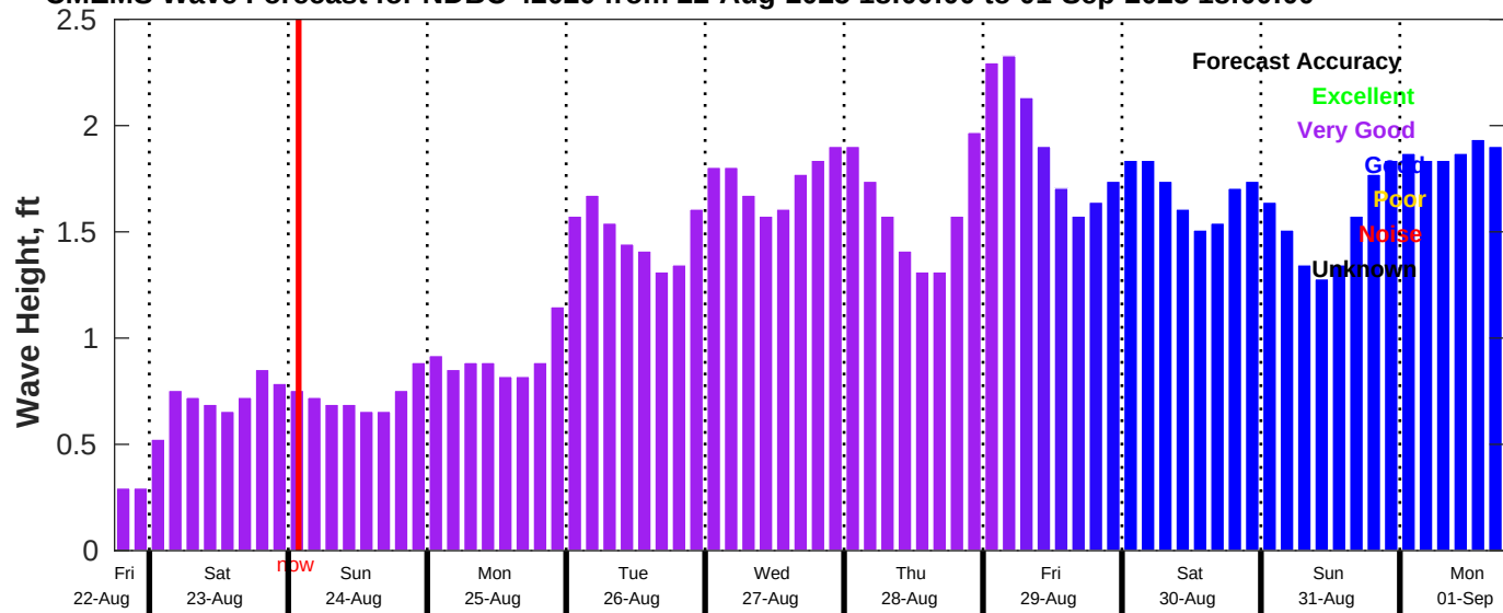
CMEMS Wave Forecast for NDBC 42020 from 22-Aug-2025 18:00:00 to 01-Sep-2025 18:00:00
