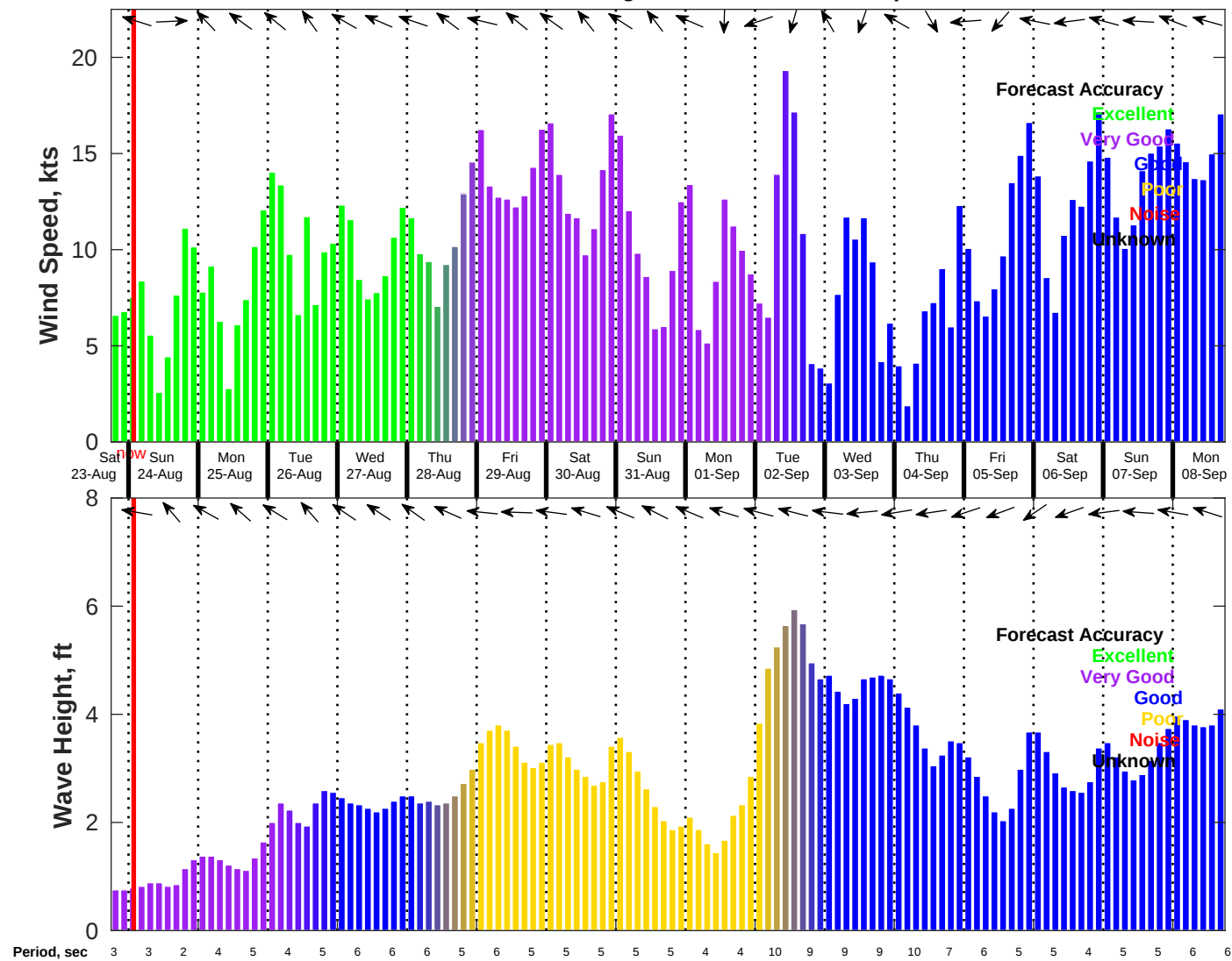
Wind & Wave Forecast for NDBC 42020 from 23-Aug-2025 18:00:00 to 08-Sep-2025 18:00:00
