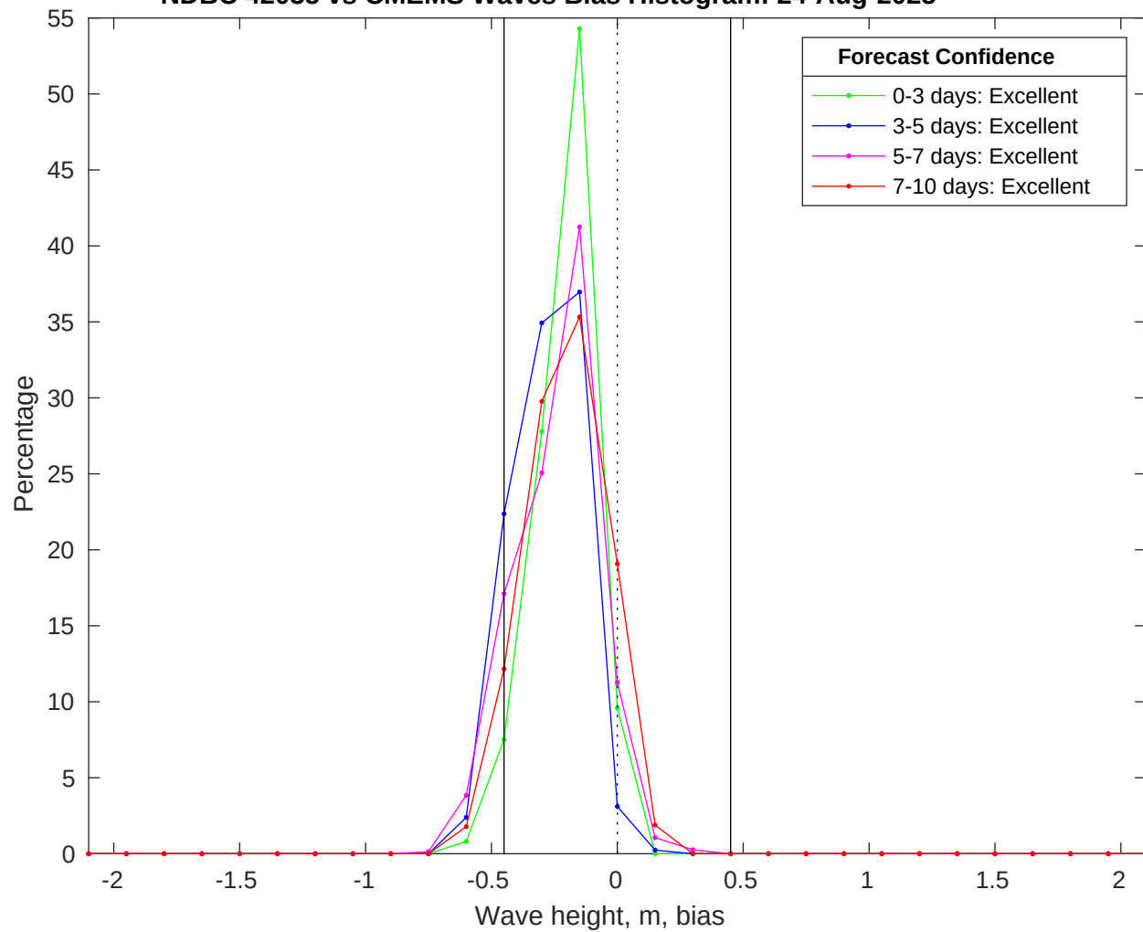
NDBC 42035 vs CMEMS Waves Bias Histogram: 24-Aug-2025
