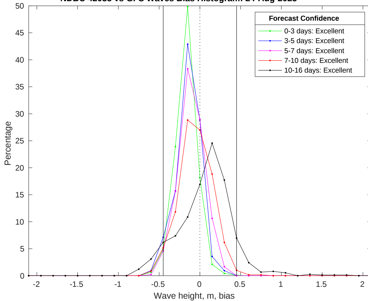
NDBC 42035 vs GFS Waves Bias Histogram: 24-Aug-2025
