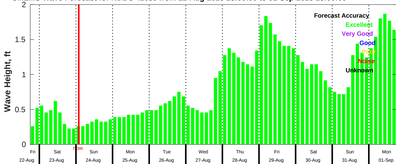
CMEMS Wave Forecast for NDBC 42035 from 22-Aug-2025 18:00:00 to 01-Sep-2025 18:00:00
