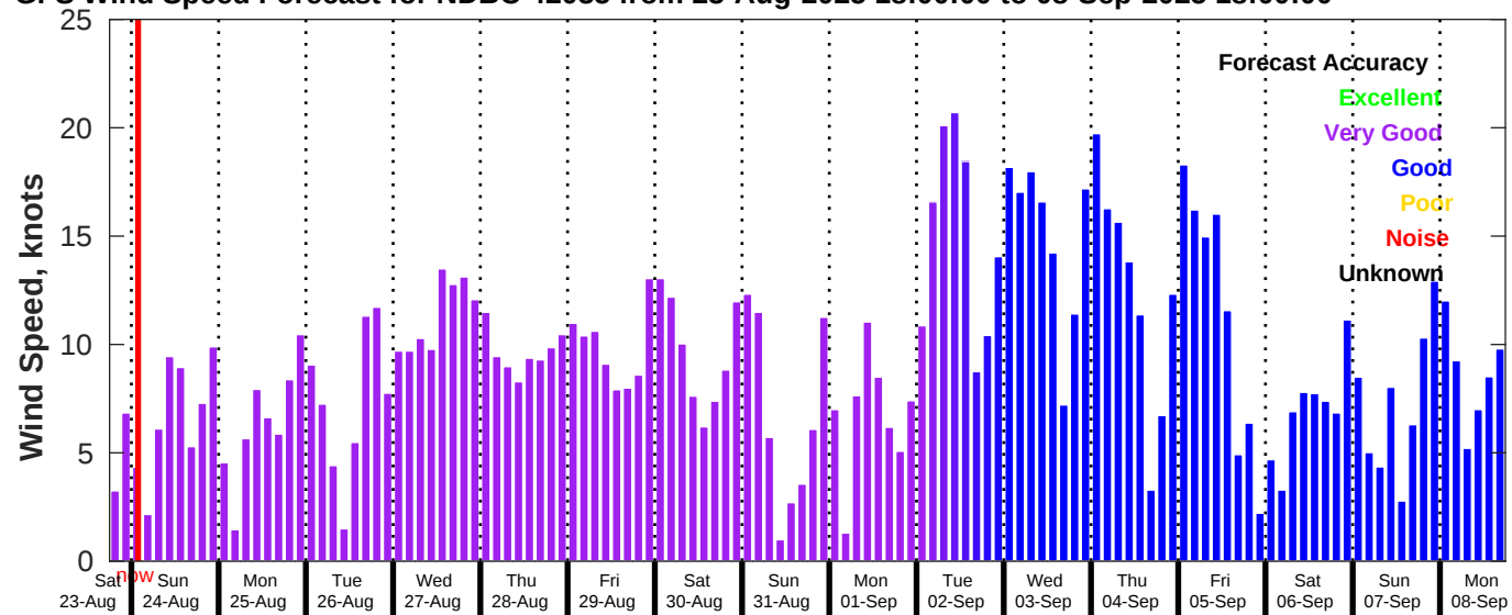
GFS Wind Speed Forecast for NDBC 42035 from 23-Aug-2025 18:00:00 to 08-Sep-2025 18:00:00
