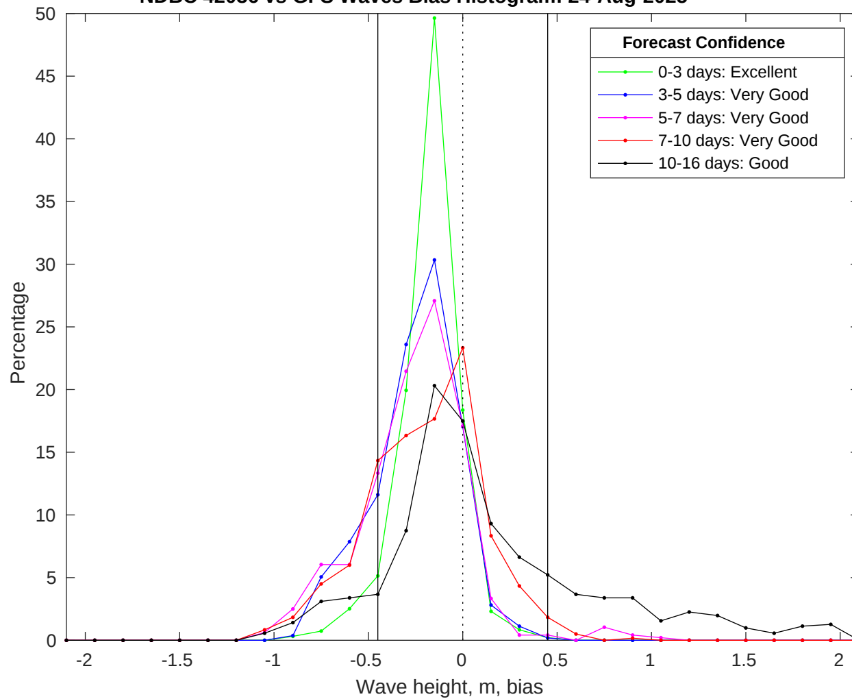
NDBC 42036 vs GFS Waves Bias Histogram: 24-Aug-2025
