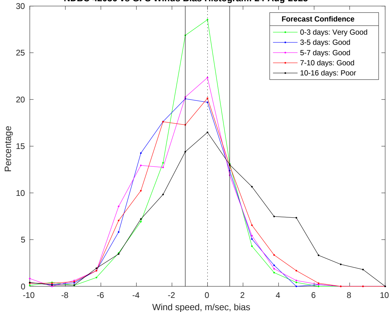
NDBC 42036 vs GFS Winds Bias Histogram: 24-Aug-2025
