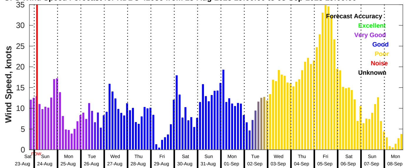
GFS Wind Speed Forecast for NDBC 42036 from 23-Aug-2025 19:00:00 to 08-Sep-2025 19:00:00
