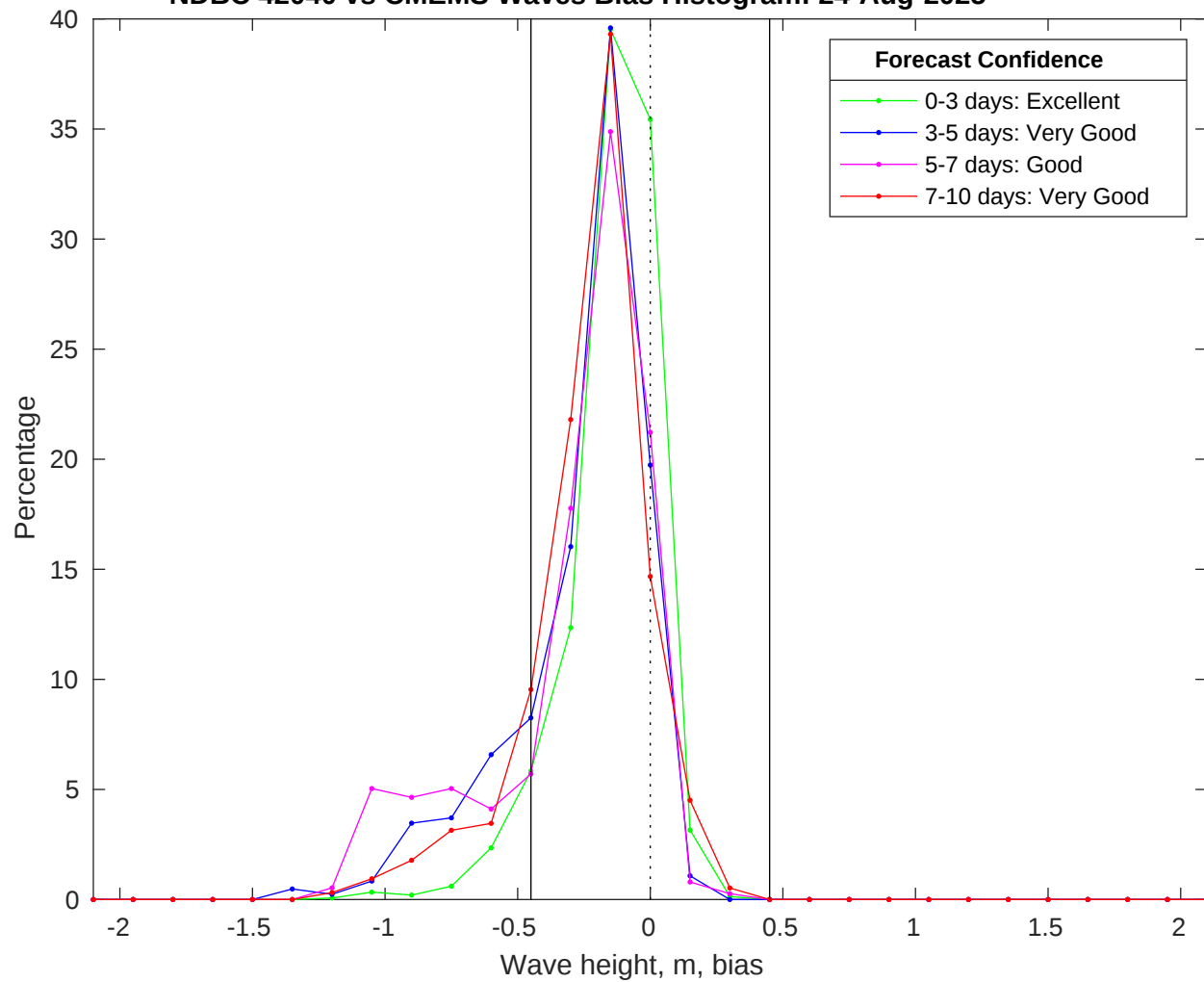
NDBC 42040 vs CMEMS Waves Bias Histogram: 24-Aug-2025
