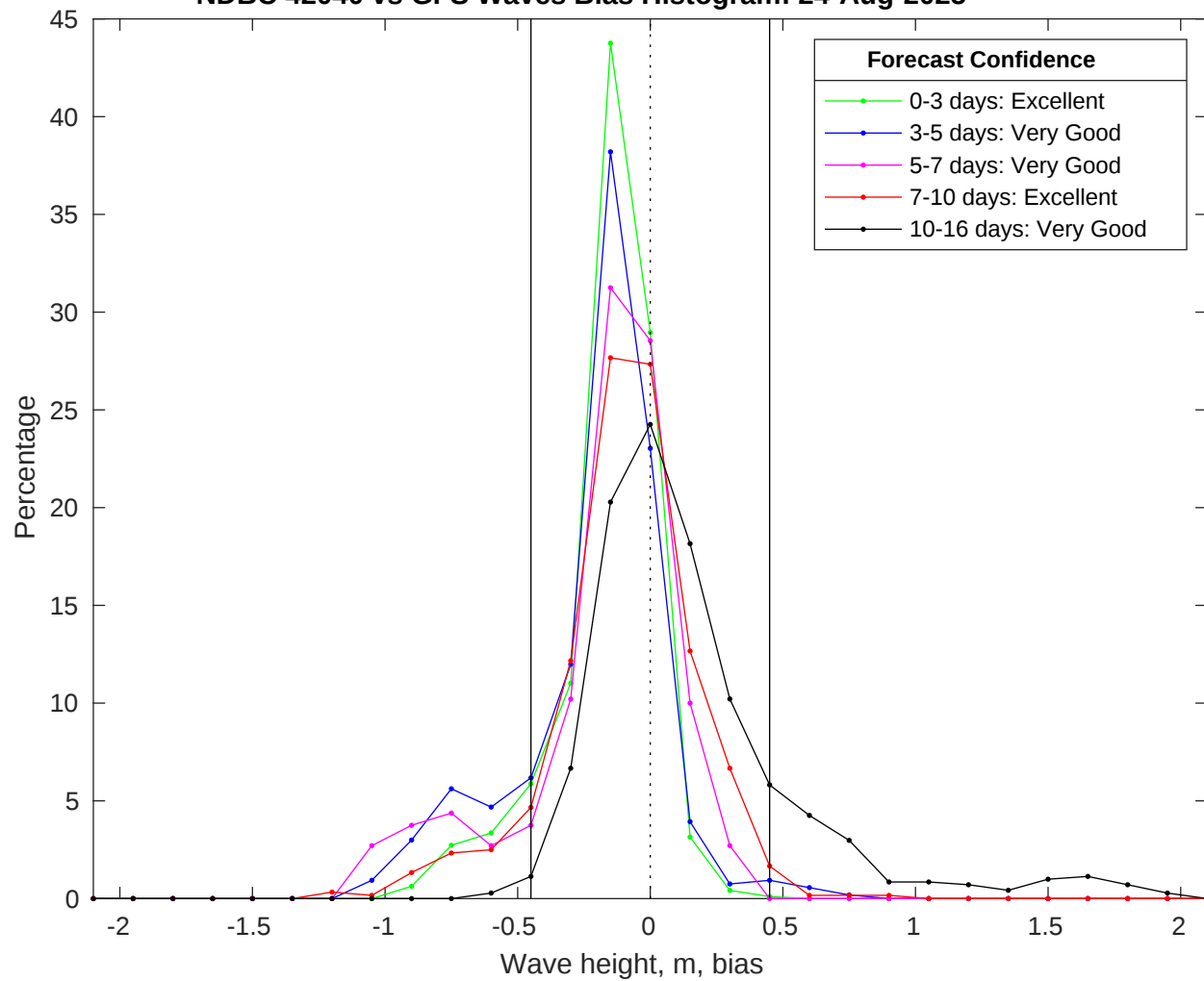
NDBC 42040 vs GFS Waves Bias Histogram: 24-Aug-2025
