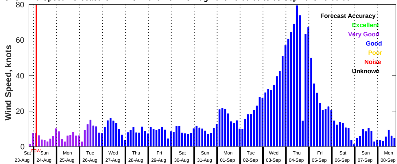
GFS Wind Speed Forecast for NDBC 42040 from 23-Aug-2025 19:00:00 to 08-Sep-2025 19:00:00
