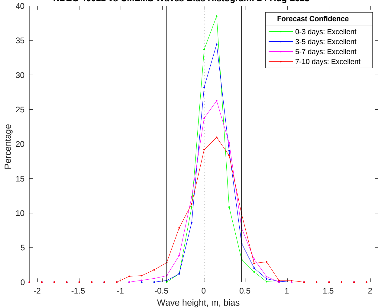
NDBC 46011 vs CMEMS Waves Bias Histogram: 24-Aug-2025
