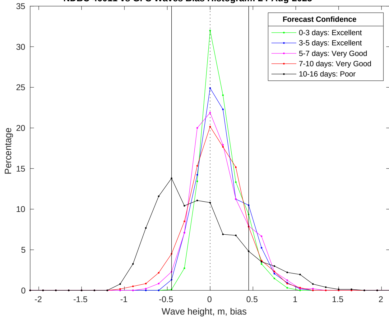
NDBC 46011 vs GFS Waves Bias Histogram: 24-Aug-2025
