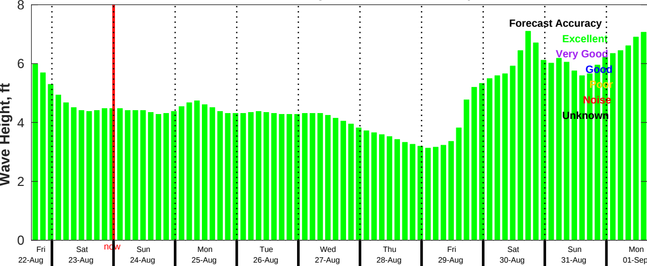
CMEMS Wave Forecast for NDBC 46011 from 22-Aug-2025 16:00:00 to 01-Sep-2025 16:00:00
