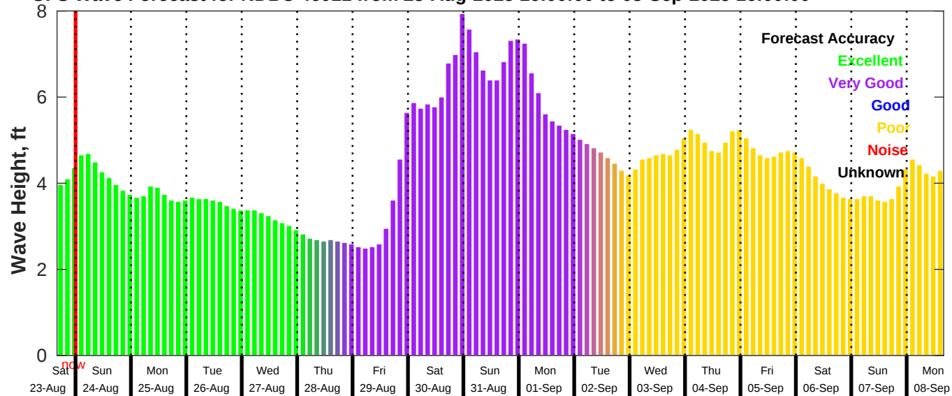
GFS Wave Forecast for NDBC 46011 from 23-Aug-2025 16:00:00 to 08-Sep-2025 16:00:00
