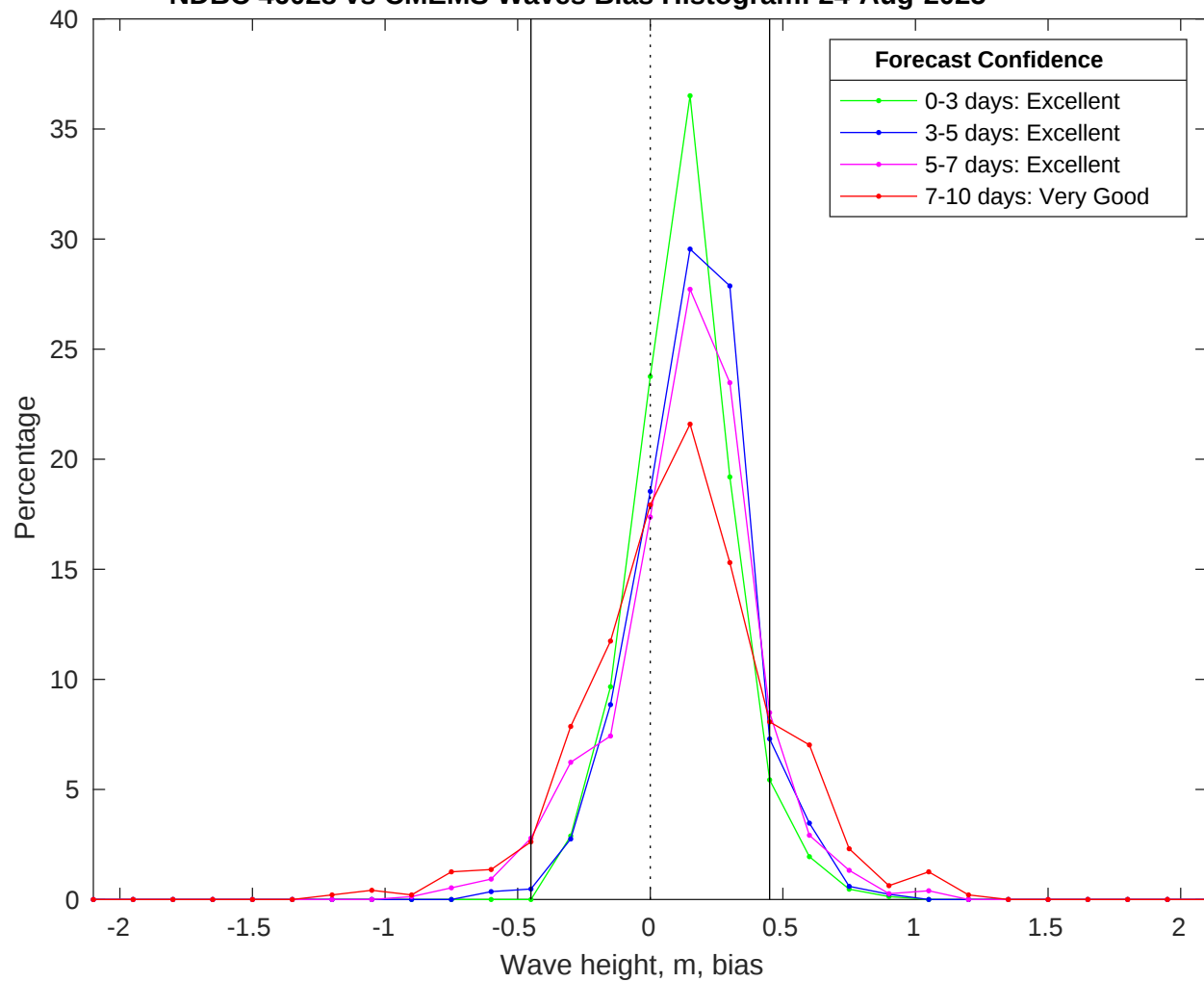
NDBC 46028 vs CMEMS Waves Bias Histogram: 24-Aug-2025
